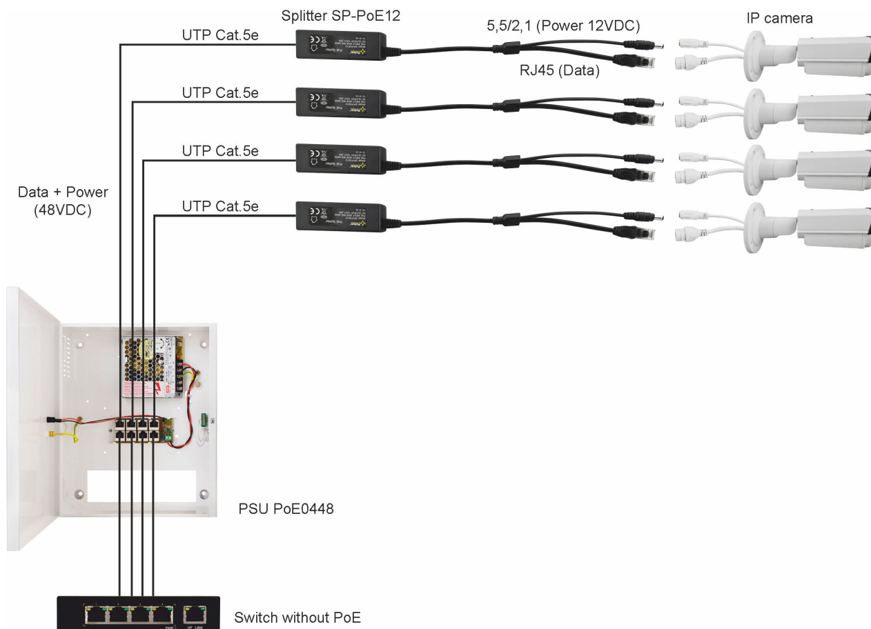
Fig. 3. Example of connection with passive PoE power supply.
